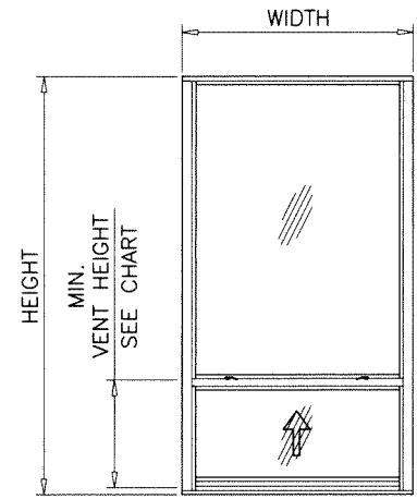
UNEQUAL LITES (ORIEL TYPE)
