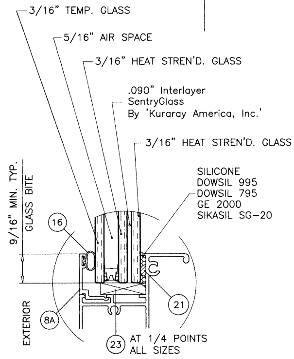
GLASS TYPE 'Bi'
